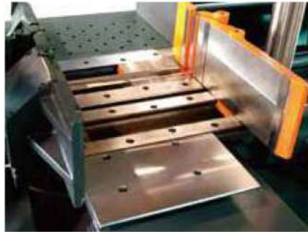
Double retracting vises
